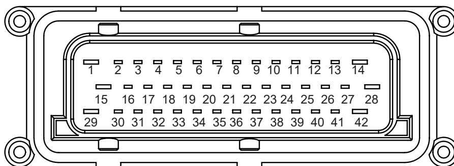
Pin assignment connector 42 Pin (1)
