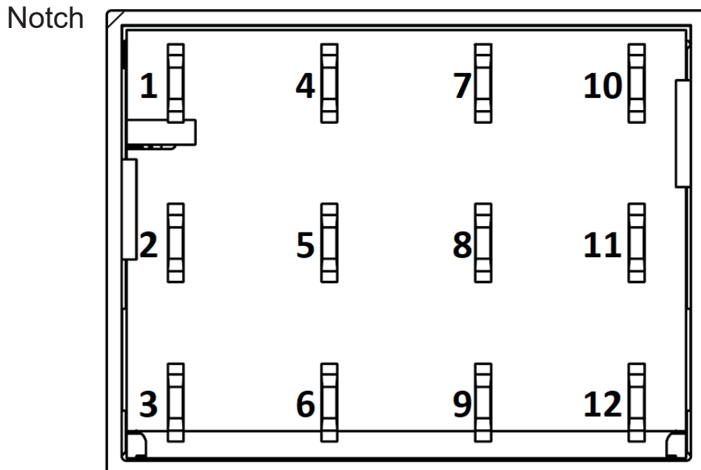
Pin assignment - bottom view
