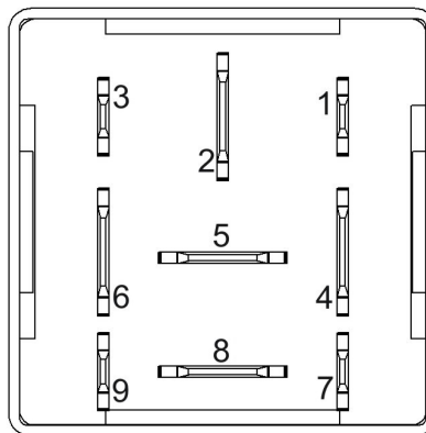
Pin assignment - bottom view
