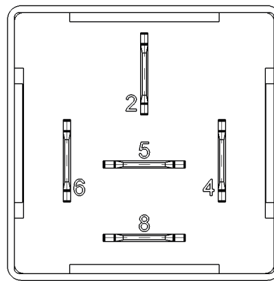
Pin assignment, bottom view
